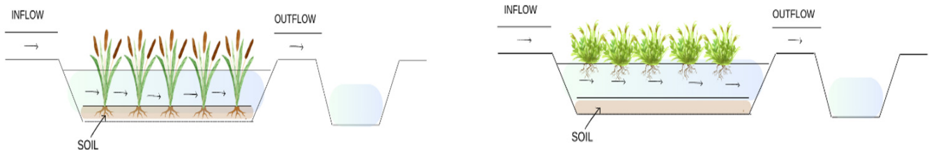
Figure 2. Free water surface wetland: free floating (top), emergent rooted plants (bottom) (based on Vymazal, 2007)
